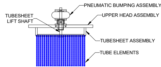
UPPER HEAD AND ELEMENT DETAIL
